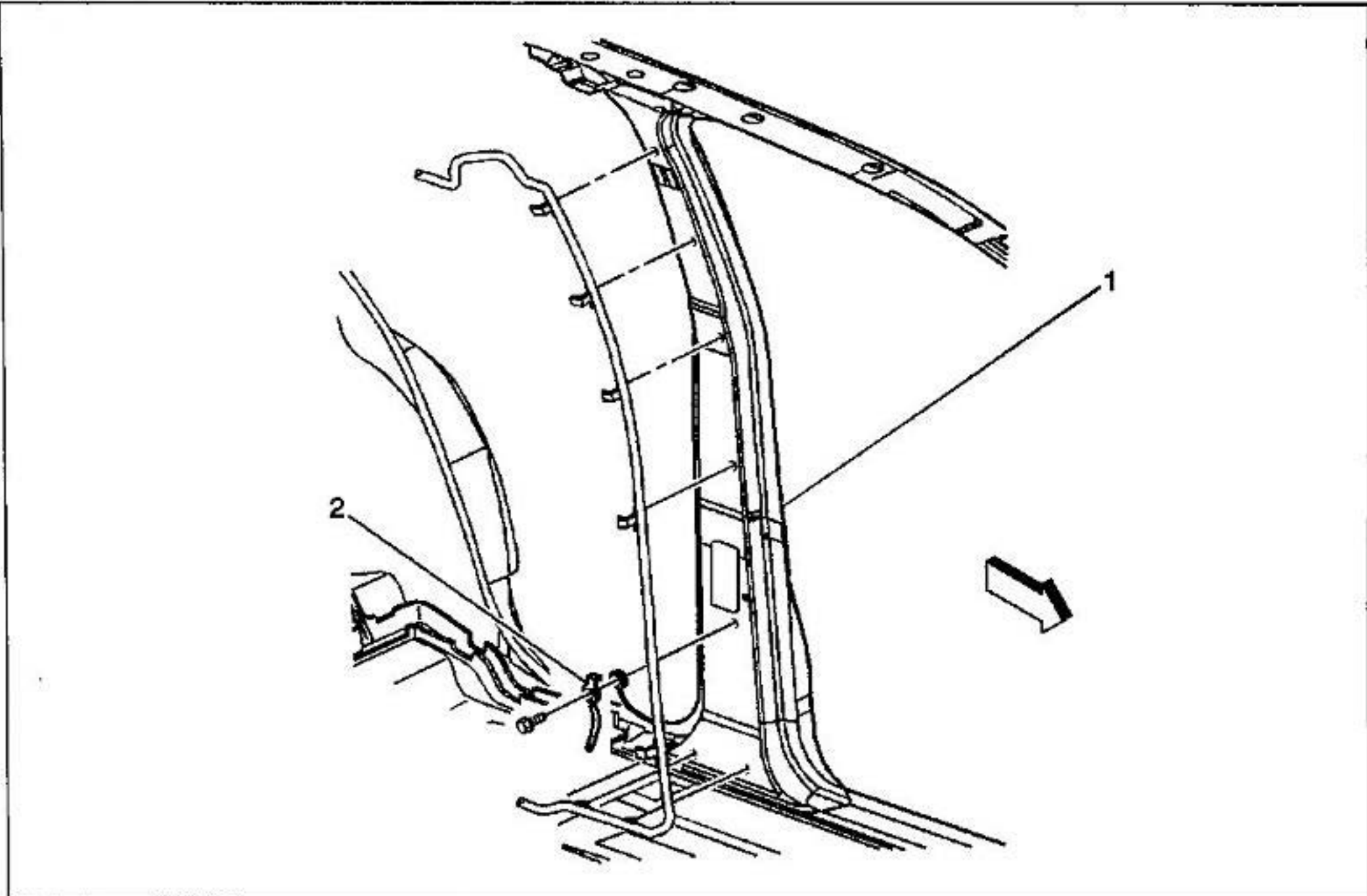
B-Pillar, Left-G302
